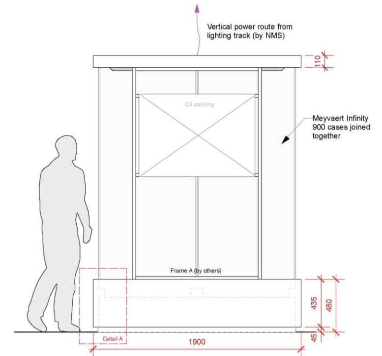
Side Elevation Table top case Scale 1:25
